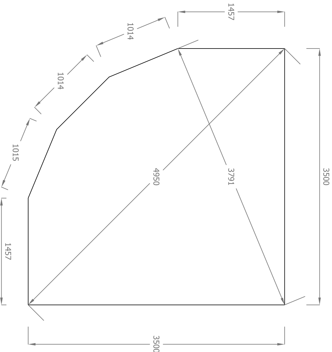
Base Plan
